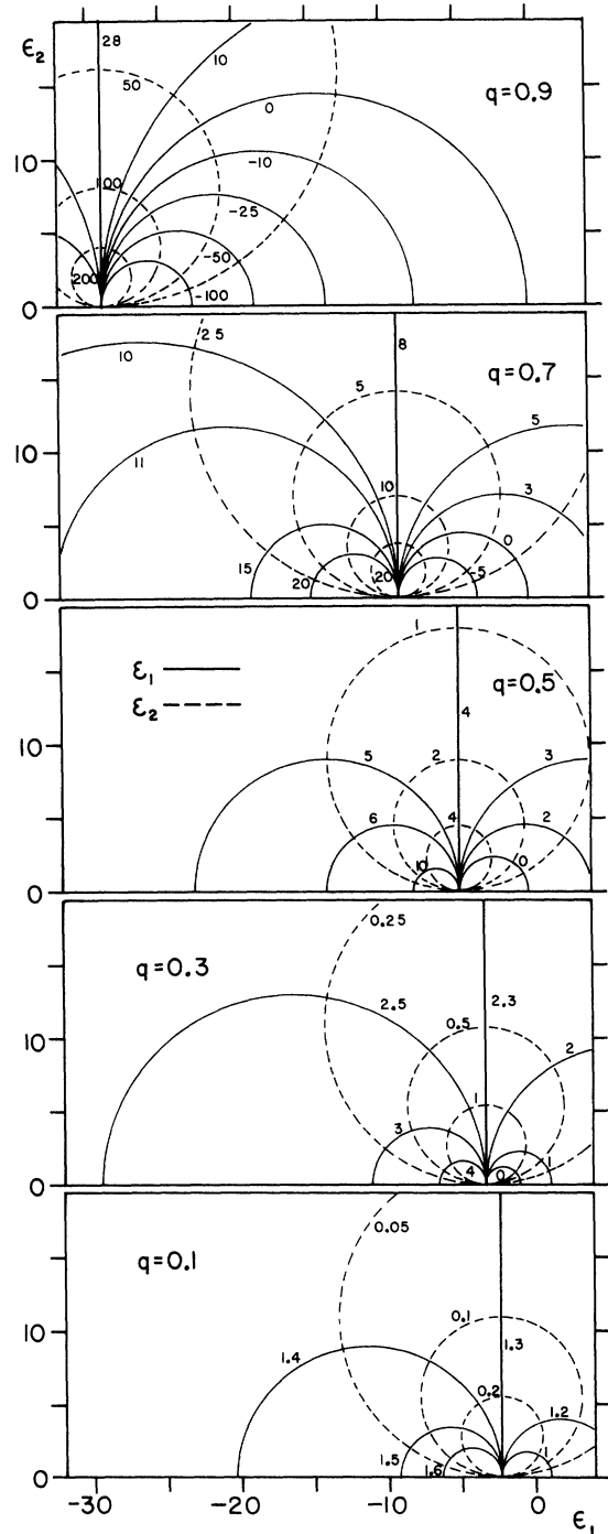
FIG. 2. Coordinate system (\delta_1, \delta_2) mapped on the Cartesian plane (\epsilon_1, \epsilon_2) for several values of q , representing the complete MG transformation according to Eqs. (5) and (7). Transformation is restricted to the physically meaningful region of \epsilon_2 \geq 0 .
